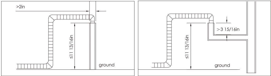
Drain-pipe installation diagram
